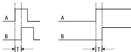
A/B time displacement when converting direction standard 2 or 3 to quadrature standard
