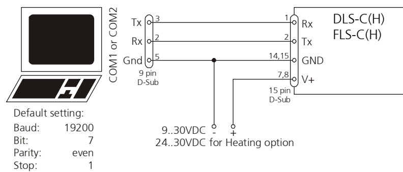
Fig. 8 Connection for DLS-C(H)/FLS-C(H) configuration
