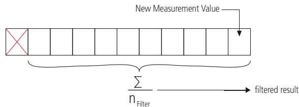
Fig. 10 Moving average filter
