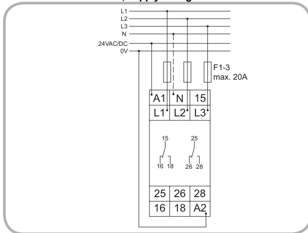
► G2PM400VSY20 24-240V, supply voltage 24V AC/DC
