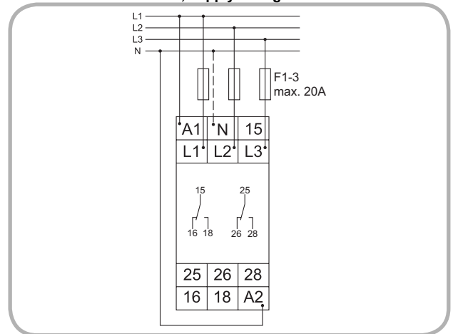
► G2PM400VSY20 24-240V, supply voltage 230V AC
