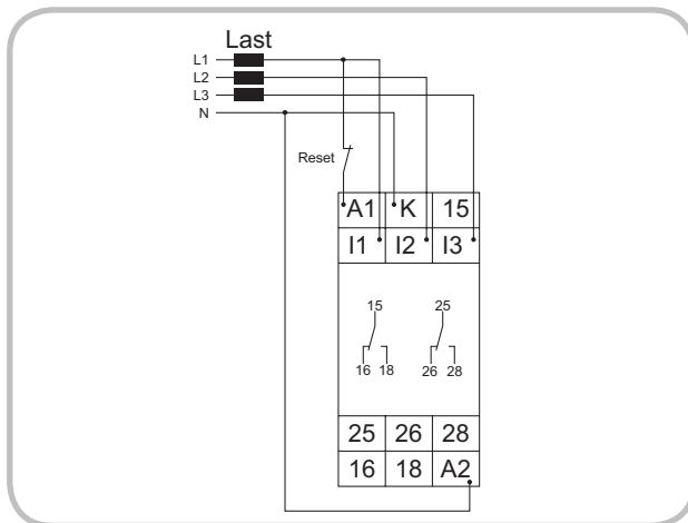
► G2JM5AL20, supply voltage 230V AC and fault latch
