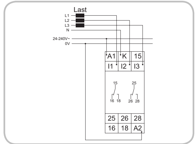
► G2JM5AL20, supply voltage 24-240V AC/DC without fault latch
