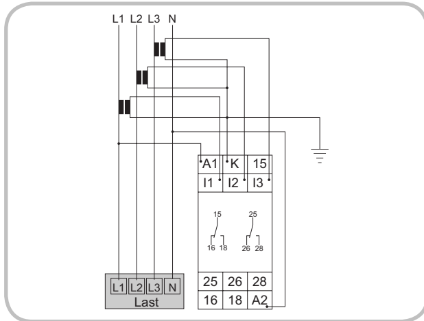
► G2JM5AL20, supply voltage 230V AC and current transformer
