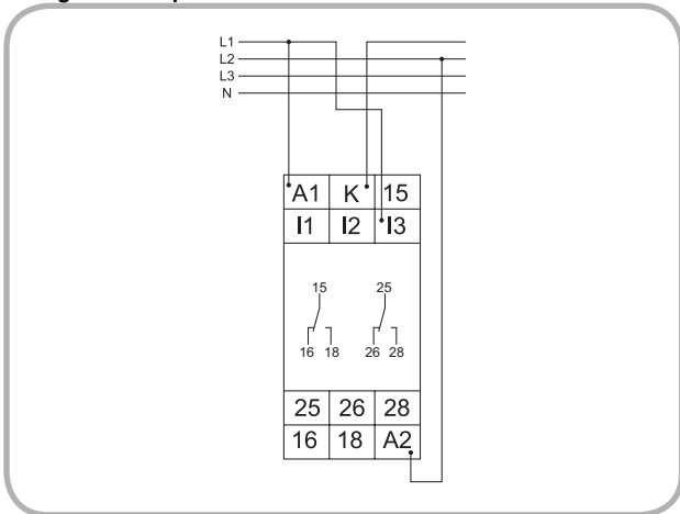
► Range 5A with power modul 400V AC without fault latch
