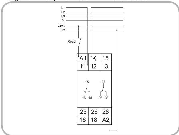
► Range 20mA with power modul 24V AC and fault latch
